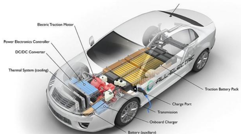
All-Electric Vehicle
